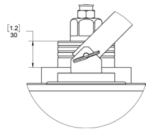
Swivel to be set 1.2" (30mm) from collar
